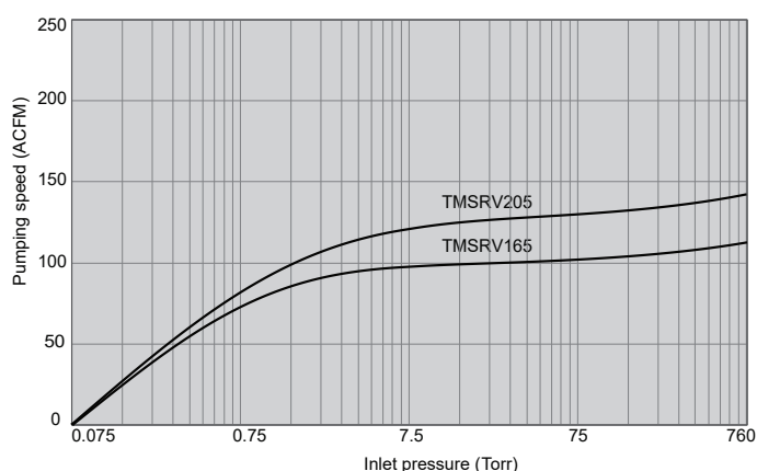
Pumping Speed
