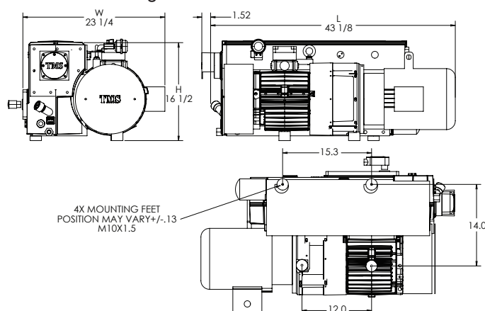
Dimensional Drawing
