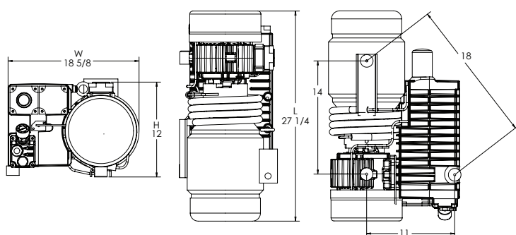
Dimensional Drawing
