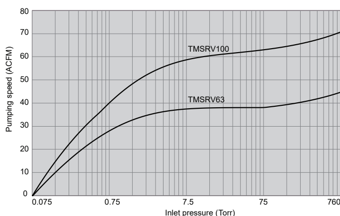
Pumping Speed
