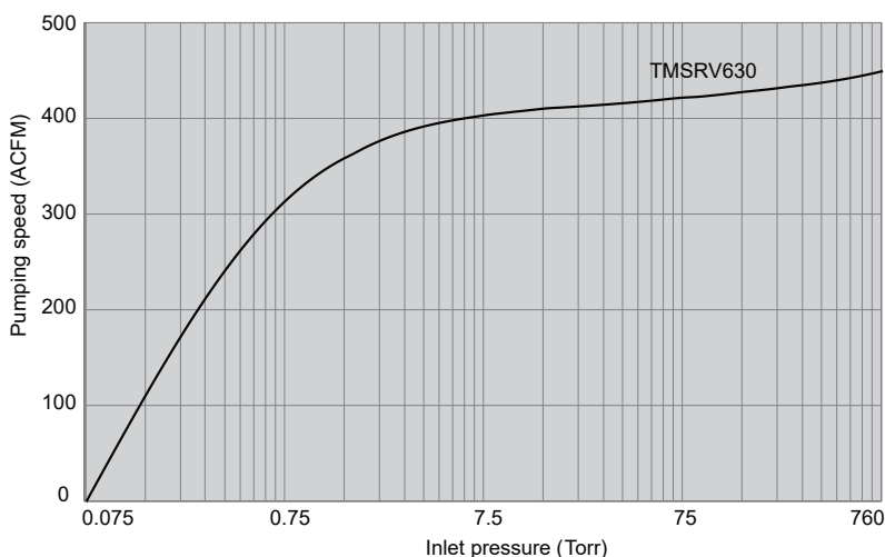
Pumping Speed
